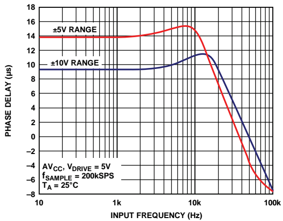
Figure 34. Analog Antialiasing Filter Phase Response
